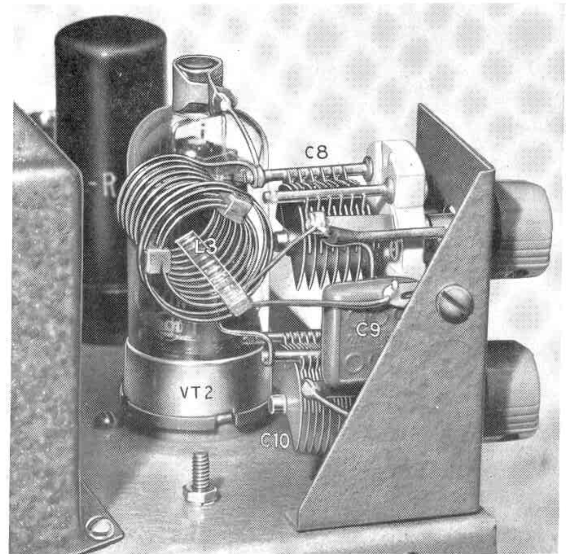
Figure 2. ST-203-A Amplifier Tank Assembly
